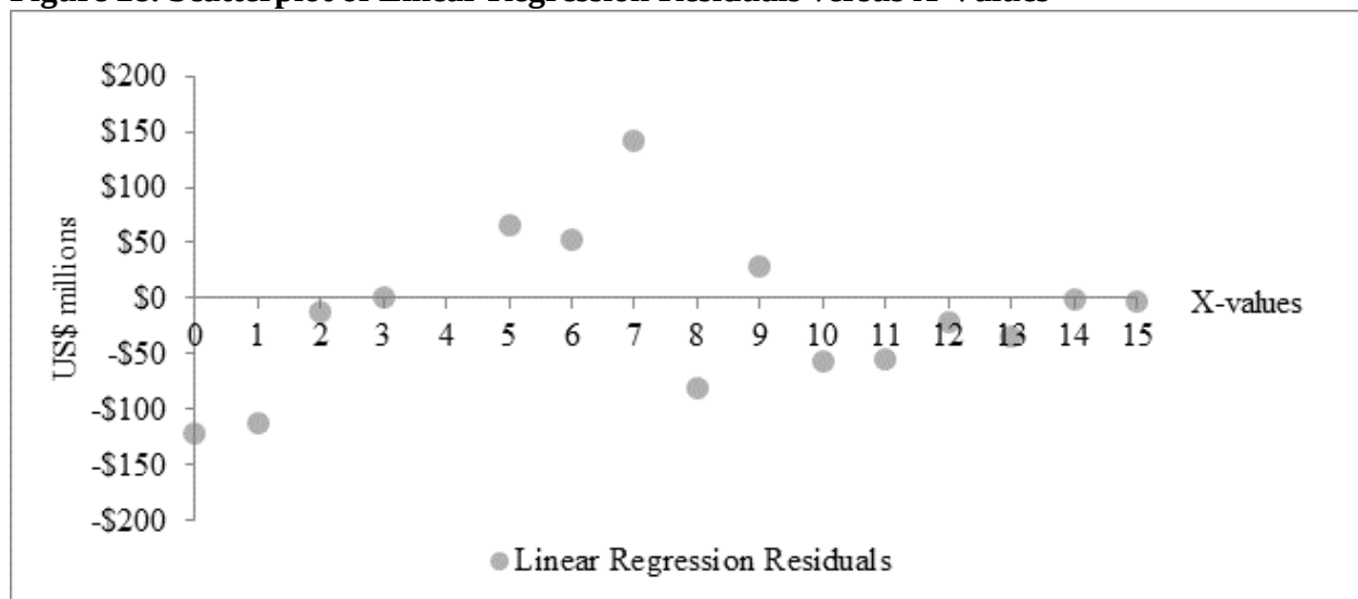
Figure 28. Scatterplot of Linear Regression Residuals versus X-Values
